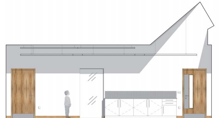
elevation D
