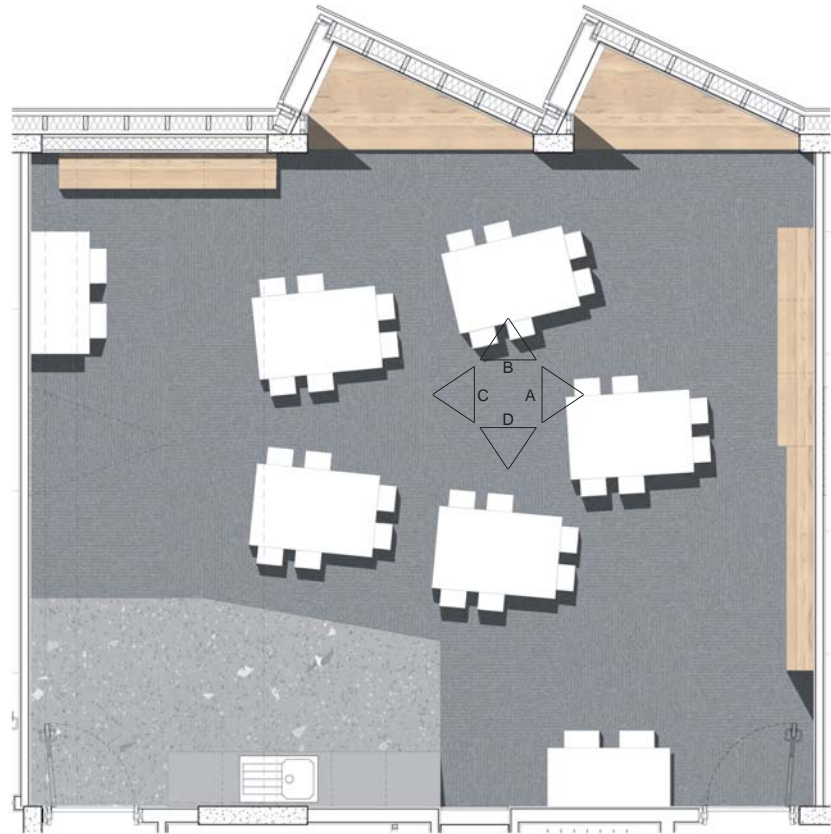
first floor class base plan
